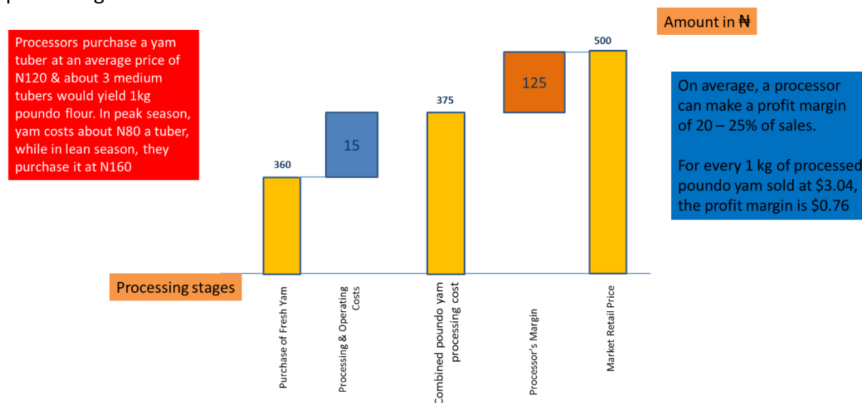
Figure 6: Processor Economics
